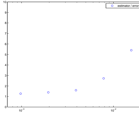
Figure 2: \eta_h/e_{h,dis}^{rot} versus h .
