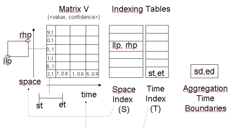
Figure 1: Storage structure of the events
